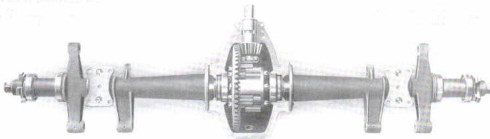
View of Rear Axle (shown in 1908) from second Swift car
