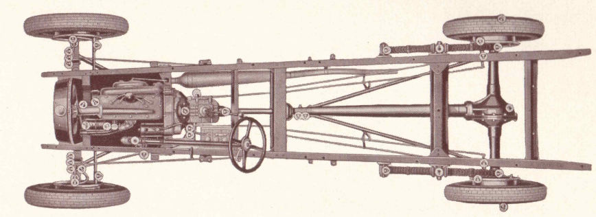
Ford Model A-A Chassis 131 1/2" (334 cm)
