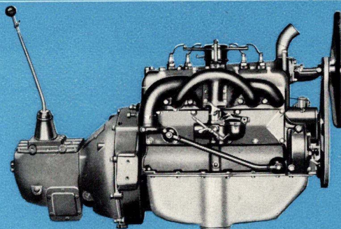
Model AA 4-cylindret Motor 4 Gear.
