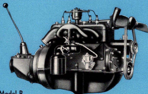
Model B 4-cyl. Motor. 3 Gear
