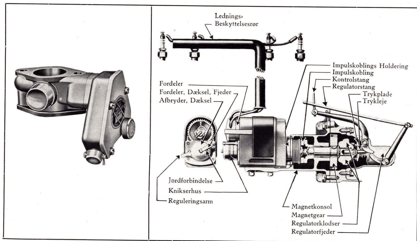
Regulator for 4-cyl. Model „B” Motor
