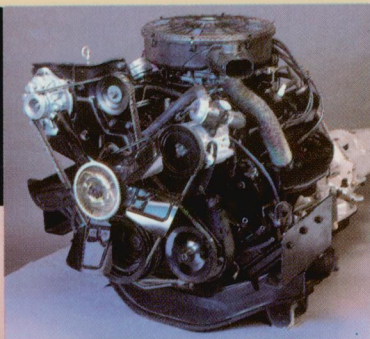
5.2-liter V-8 engine with electronic fuel injection.
